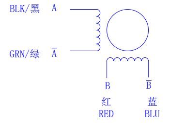
励磁顺序(2相励磁) EXCITING SEQUENCE (TWO PHASE)
