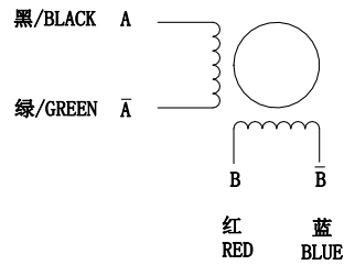
励磁顺序(2相励磁) EXCITING SEQUENCE(TWO PHASE)
