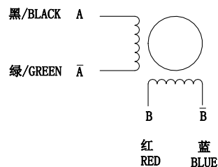
励磁顺序(2相励磁) EXCITING SEQUENCE(TWO PHASE)
